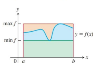
(e) Max-Min Inequality:
