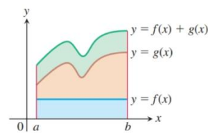
(c) Sum: (areas add)
