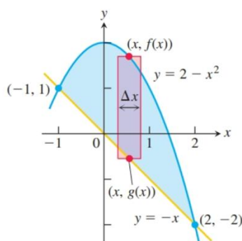
FIGURE 5.28 The region in Example 5 with a typical approximating rectangle from a Riemann sum.
