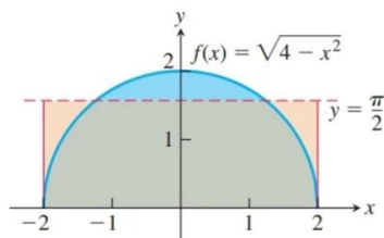
FIGURE 5.15 The average value of f(x) = \sqrt{4 - x^2} on [-2, 2] is \pi/2 (Example 7). The area of the rectangle shown here is 4 \cdot (\pi/2) = 2\pi , which is also the area of the semicircle.
